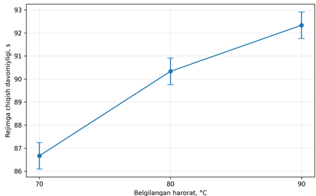
Figure 2. Relationship between the set temperature of the heating surface and the time required to reach the operating regime.
