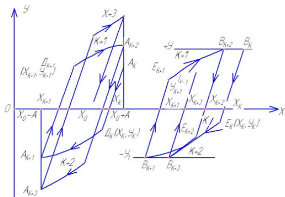
Figure 14. Cyclically unstable hysteresis
