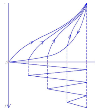
Figure 16. Hysteresis branches
