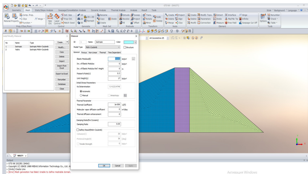
3-rasm. To'g'onning berilgan chizmasiga asosan uning 3D-modeli GTS NX dasturidagi natijalari
